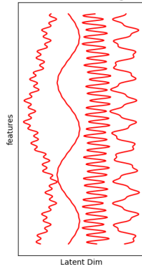
Bases ( B ) after ICA mixing matrix
